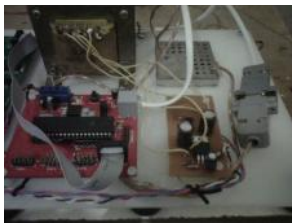
Gambar 14: Modul Pengirim Tampak Samping
