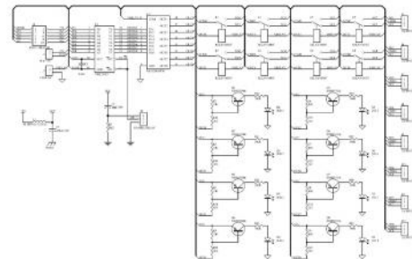
Gambar 8: Rangkaian Relay
