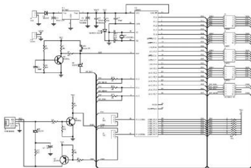
Gambar 7: Rangkaian Minimum Sistem AT89S51
